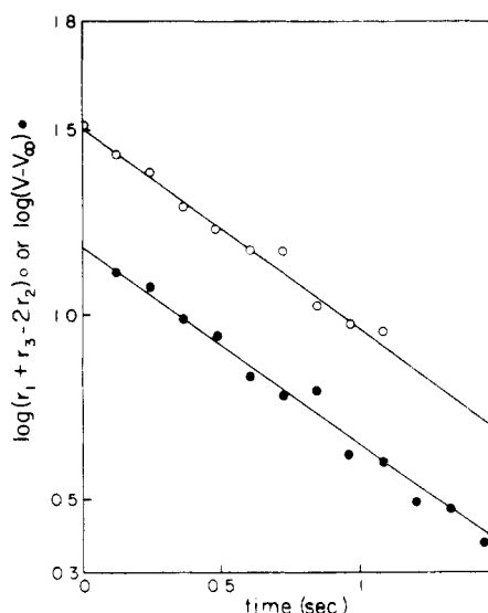
FIG. 1.—Determination of the first-order rate constant for the acylation of \alpha -chymotrypsin by p -nitrophenyl acetate at pH 7.8 at 25.0° in 4% acetonitrile-water. S_0 = 10.23 \times 10^{-4} M; E_0 = 5.78 \times 10^{-5} M.
